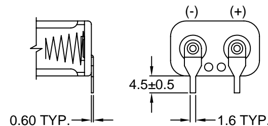
PDSN-22D PCB PINS
