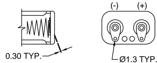
PDSN-22C SOLDER LUGS
