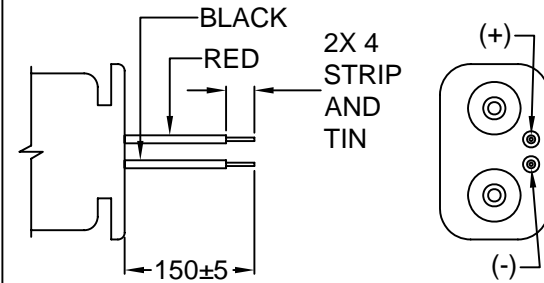
PDSN-22A WIRE LEADS
