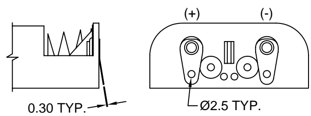
PDSN-14C SOLDER LUGS
