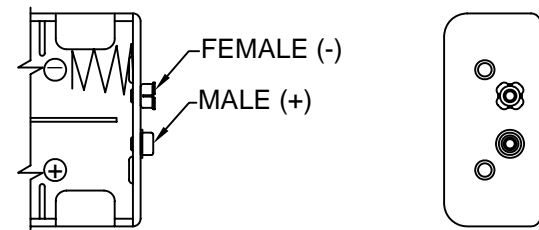
PDSN-28-3B SNAP TERMINAL
