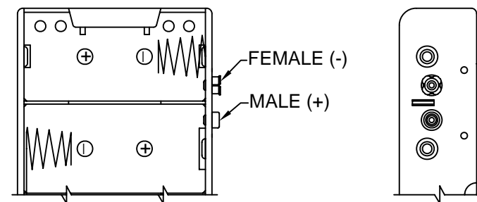
PDSN-14-2B SNAP TERMINAL
