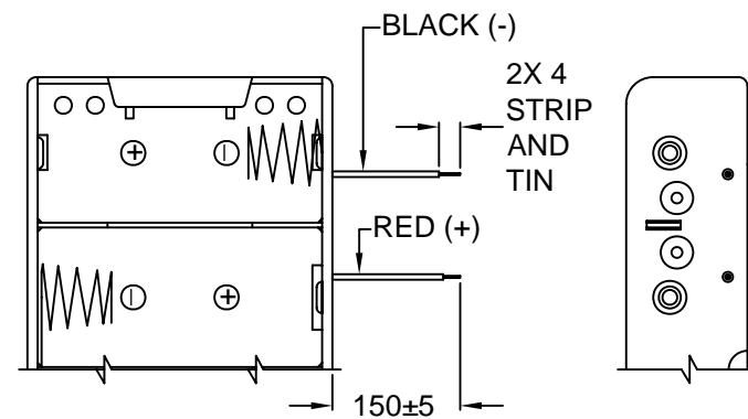
PDSN-14-2A WIRE LEADS
