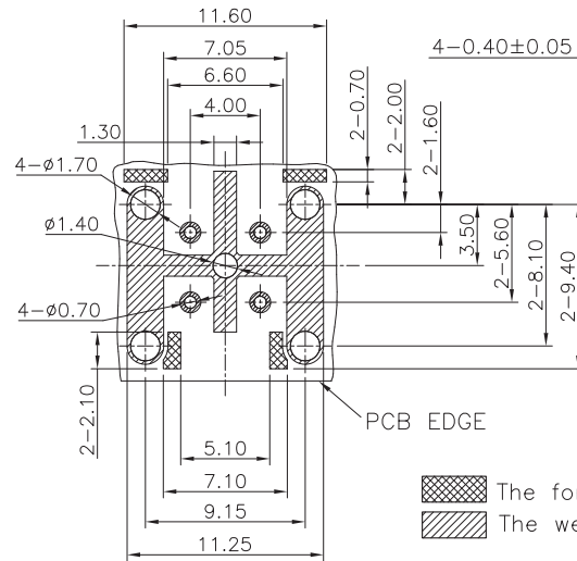
RECOMMENDED PCB LAYOUT TOP VIEW (TOLRANCE: \pm 0.05 )
